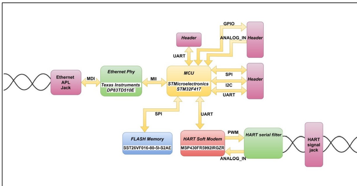
Block Diagram
